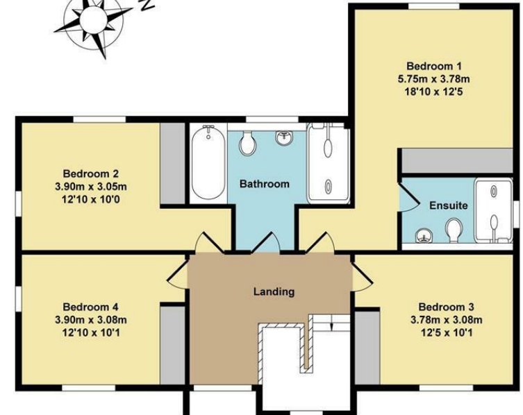
First Floor Approx. Floor Area 84.90 Sq.M. (914 Sq.Ft.)
